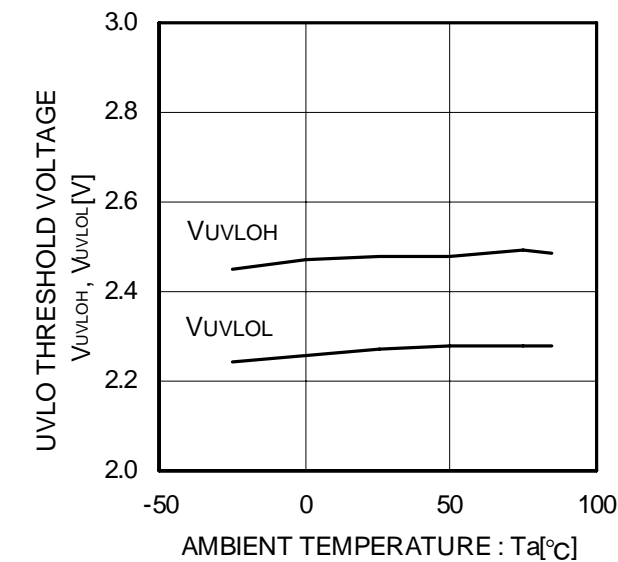
Figure 17. UVLO threshold voltage
