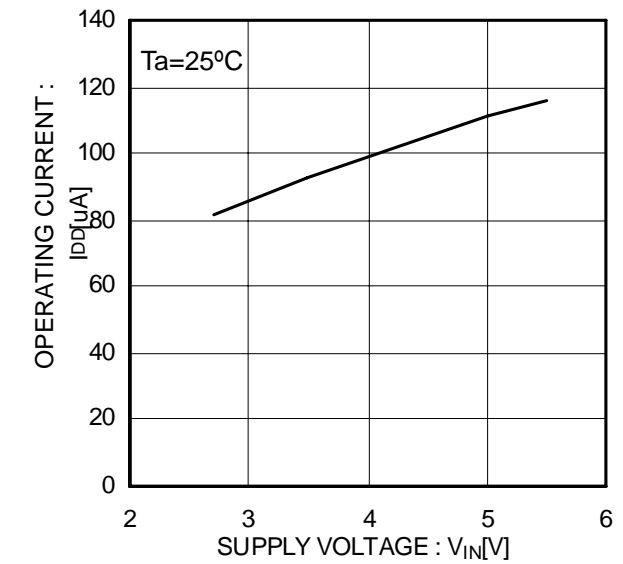
Figure 49. Operating current EN,/EN Enable
