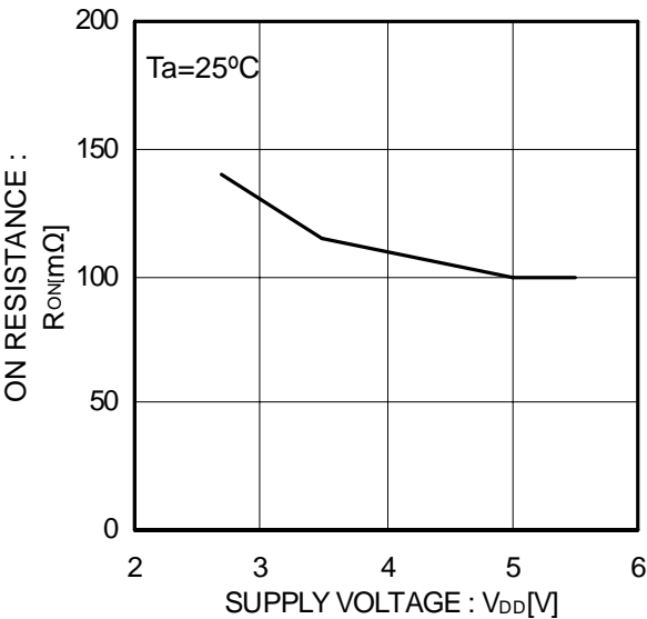
Figure 57. ON resistance
