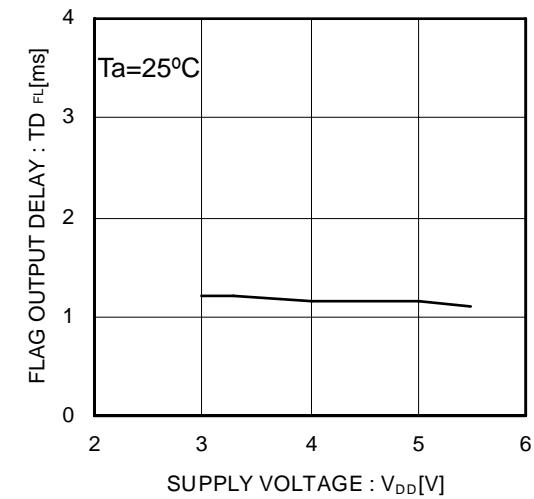
Figure 45. Flag output delay
