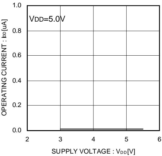
Figure 24. Operating current CTRL Disable
