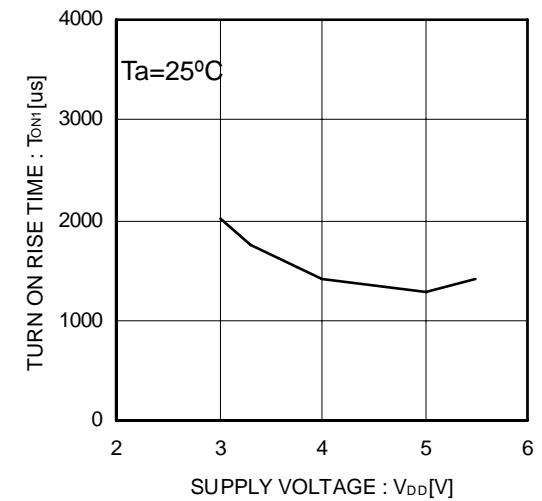
Figure 33. Output rise time
