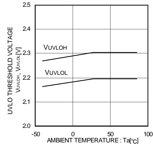
Figure 69. UVLO threshold voltage
