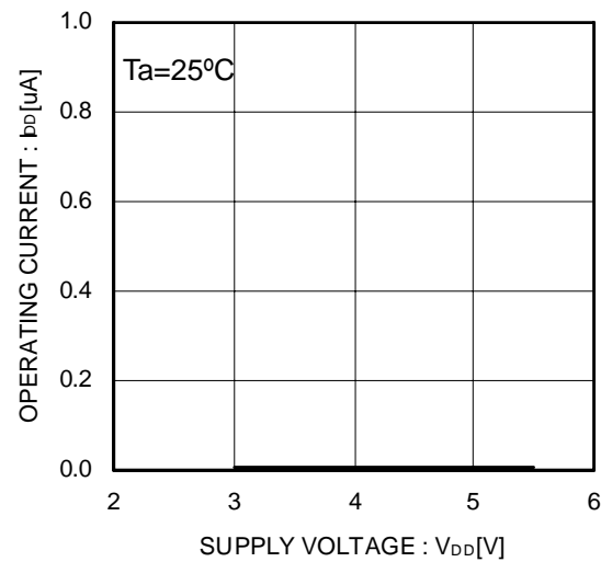
Figure 47. Operating current CTRL Disable
