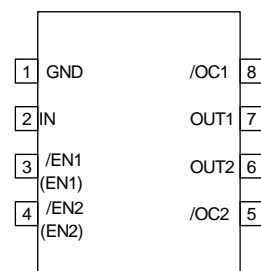
BD20xxAFJ Series TOP VIEW
