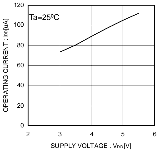
Figure 25. Operating current
