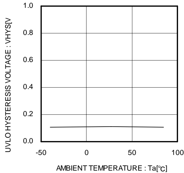
Figure 70. UVLO hysteresis voltage
