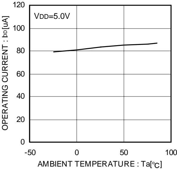
Figure 4. Operating current
