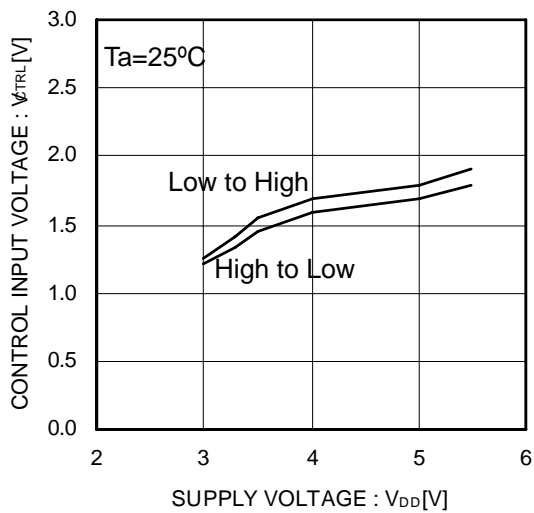
Figure 29. CTRL input voltage (BD6517F)
