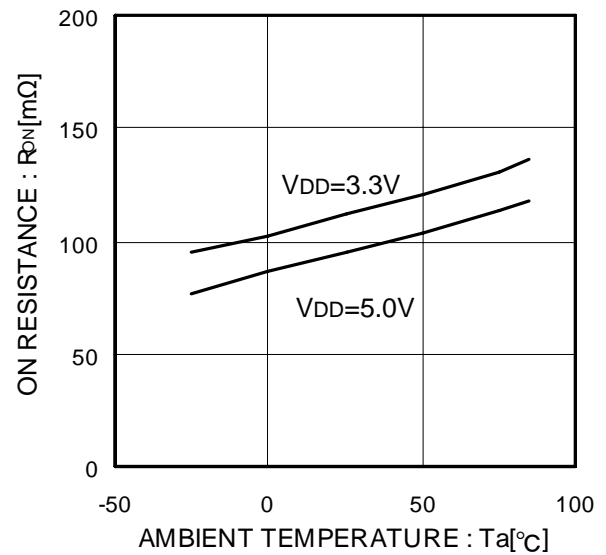
Figure 8. ON resistance
