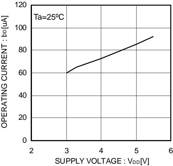
Figure 3. Operating current
