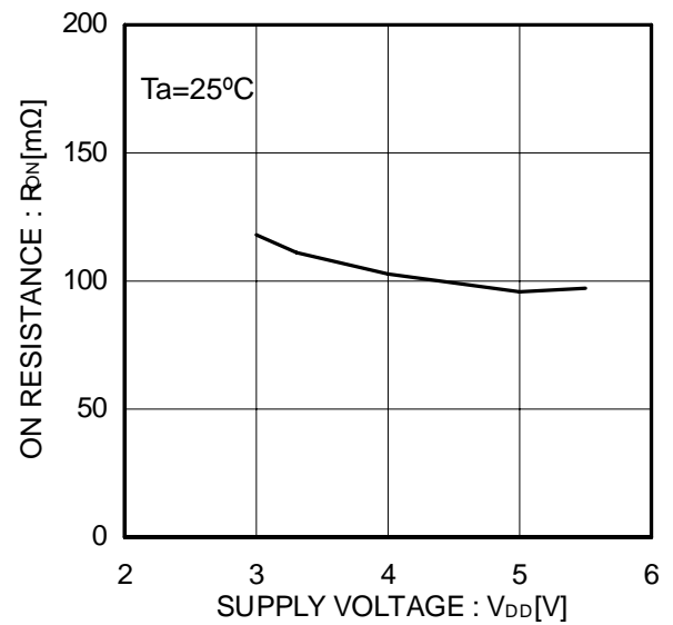
Figure 7. ON resistance
