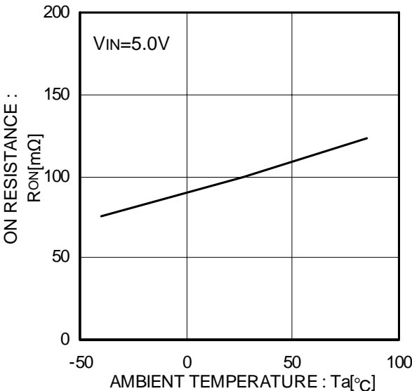
Figure 58. ON resistance
