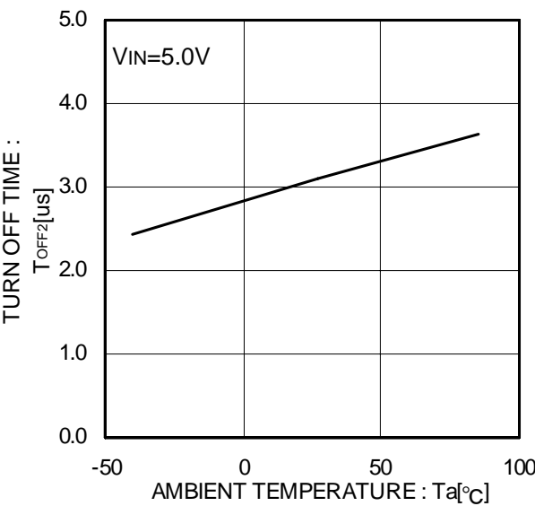
Figure 68. Output turn off time
