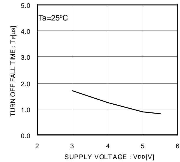
Figure 13. Output fall time
