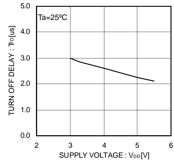
Figure 15. Output fall delay time
