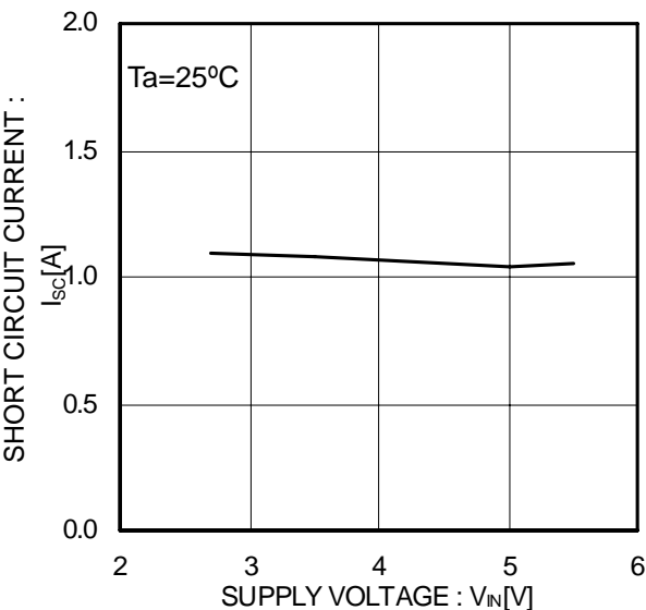
Figure 59. Output current at short-circuit
