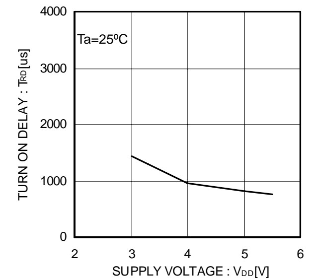
Figure 11. Output rise delay time
